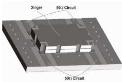
Figure 3: Component Placement
