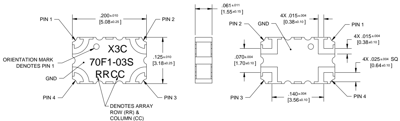
Dimensions are in Inches [Millimeters] X3C70F1-03S Mechanical Outline
