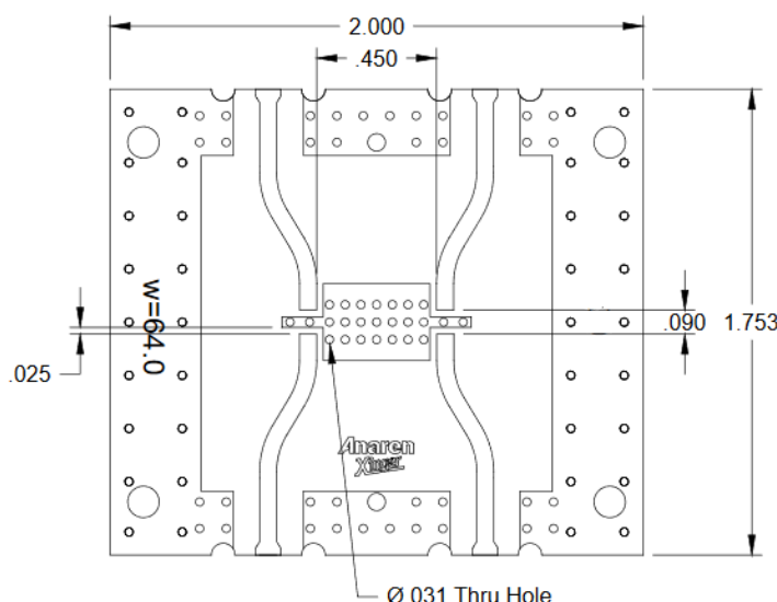
3dB Coupler Test Board
