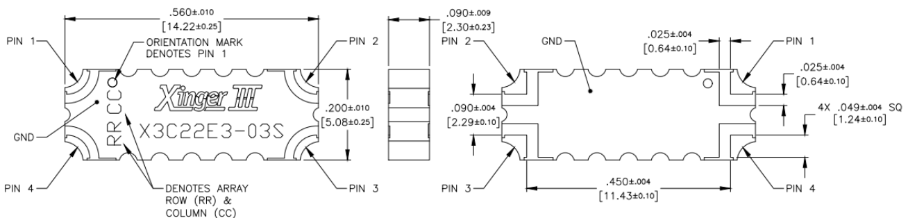
Dimensions Are in Inches [Millimeters] X3C22E3-03S Mechanical Outline
