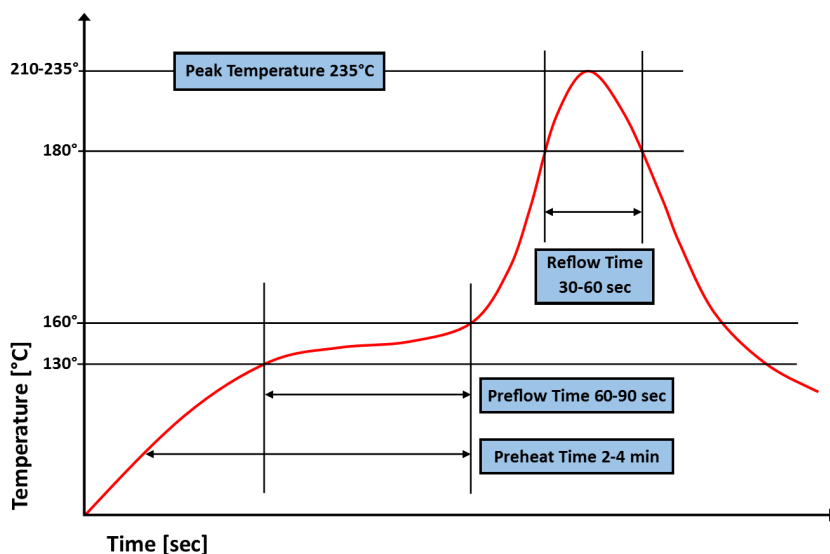
Figure 5 – Low Temperature Solder Reflow Thermal Profile
