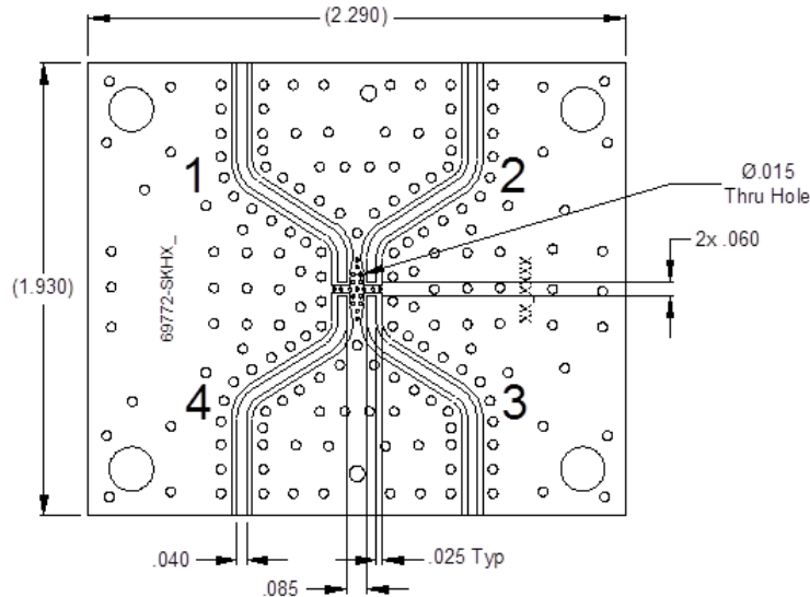
2dB- 5dB Coupler Test Board
