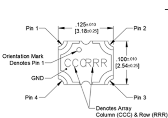
Dimensions are in Inches [Millimeters] X4C30K1-05S Mechanical Outline
