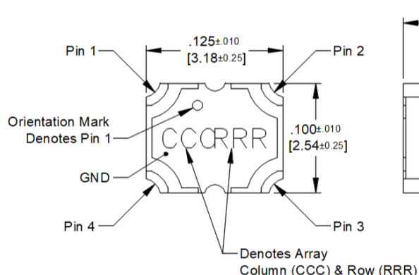
Dimensions are in Inches [Millimeters] Mechanical Outline
