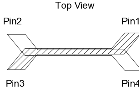
2dB Coupler Pin Configuration
