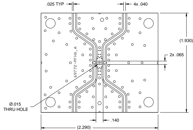
2dB - 5dB Test Board
