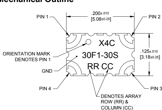
Dimensions are in Inches [Millimeters] X4C30F1-30S Mechanical Outline
