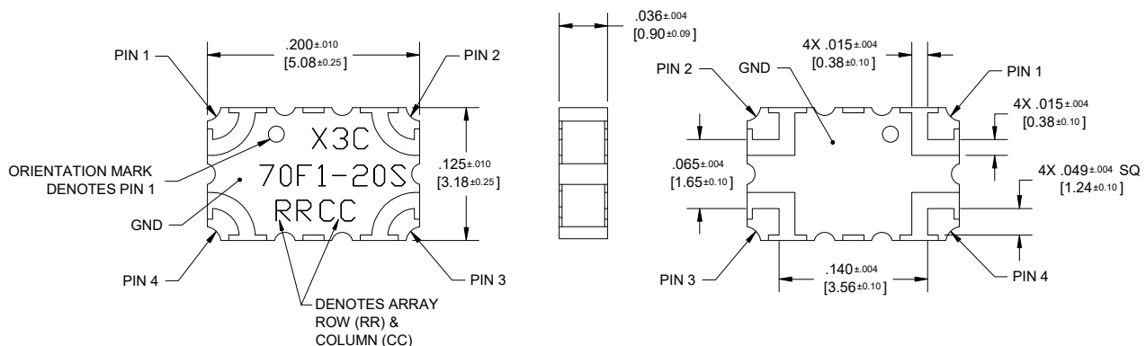
Dimensions are in Inches [Millimeters] X3C70F1-20S Mechanical Outline
