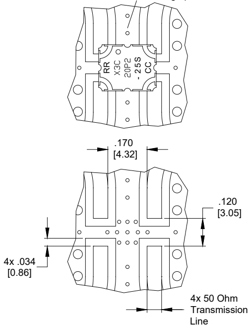
Dimensions are in Inches [Millimeters] X3C20P2-25S Mounting Footprint
