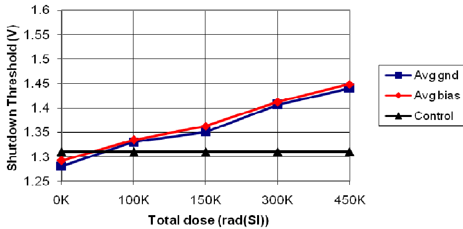
MSK5826KRH Shutdown Threshold vs. Total Dose
