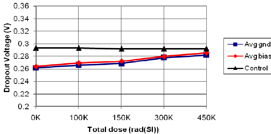
MSK5826KRH Dropout Voltage vs. Total Dose
