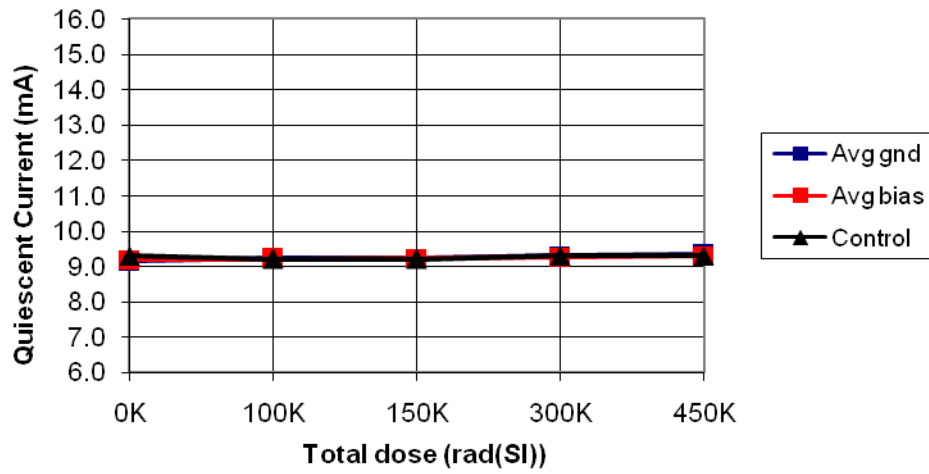
MSK5826RH Quiescent Current vs. Total Dose
