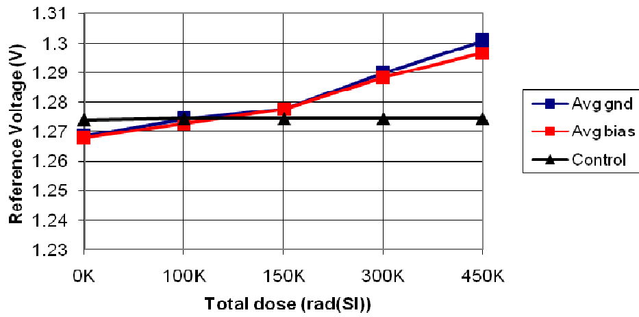
MSK5826KRH Reference Voltage vs. Total Dose
