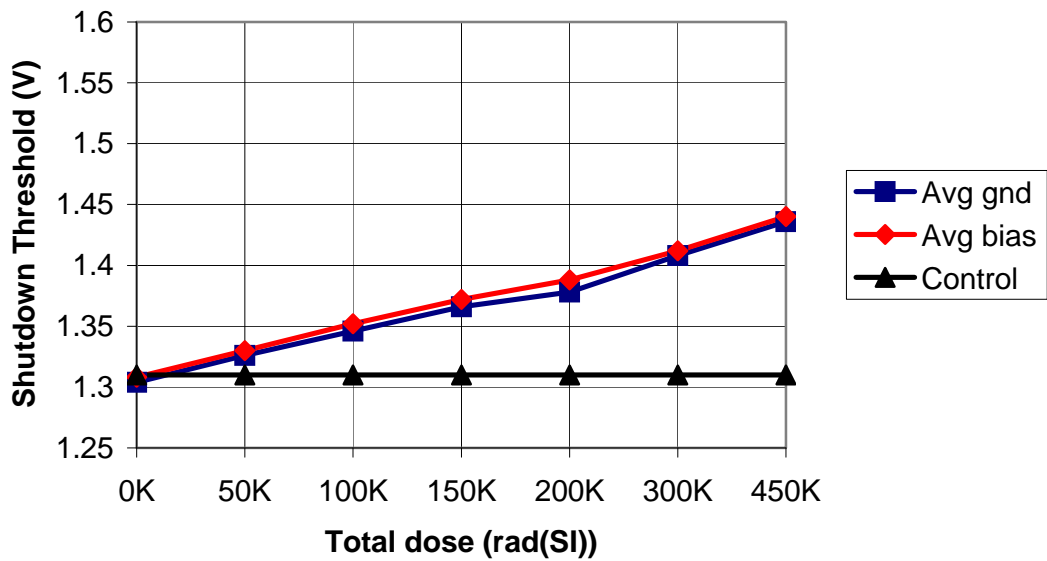
MSK5826RH Shutdown Threshold vs. Total Dose
