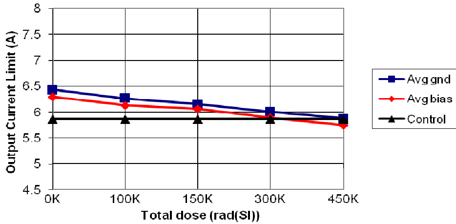
MSK5826KRH Output Current Limit vs. Total Dose
