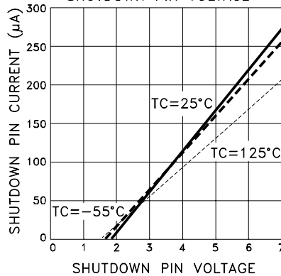
SHUTDOWN PIN CURRENT vs. SHUTDOWN PIN VOLTAGE
