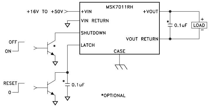
Active high shutdown and latch reset. 10mS latch off delay.
