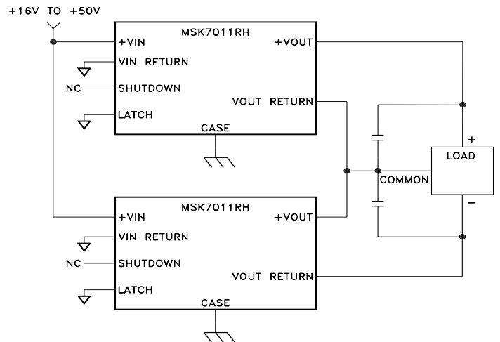
Split +/- Power Supply
